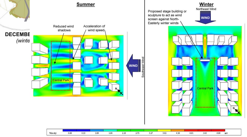
Figure 4.4 Example Computer Simulation Wind Flow
