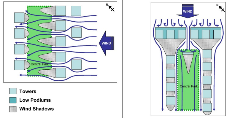
Figure 4.3 Guiding Principles for Wind Flow
